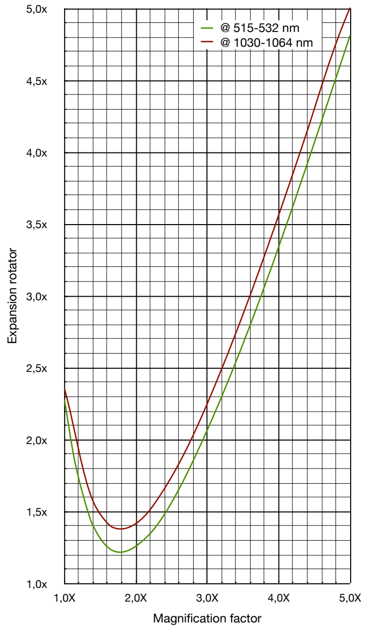
Magnification adjustment
